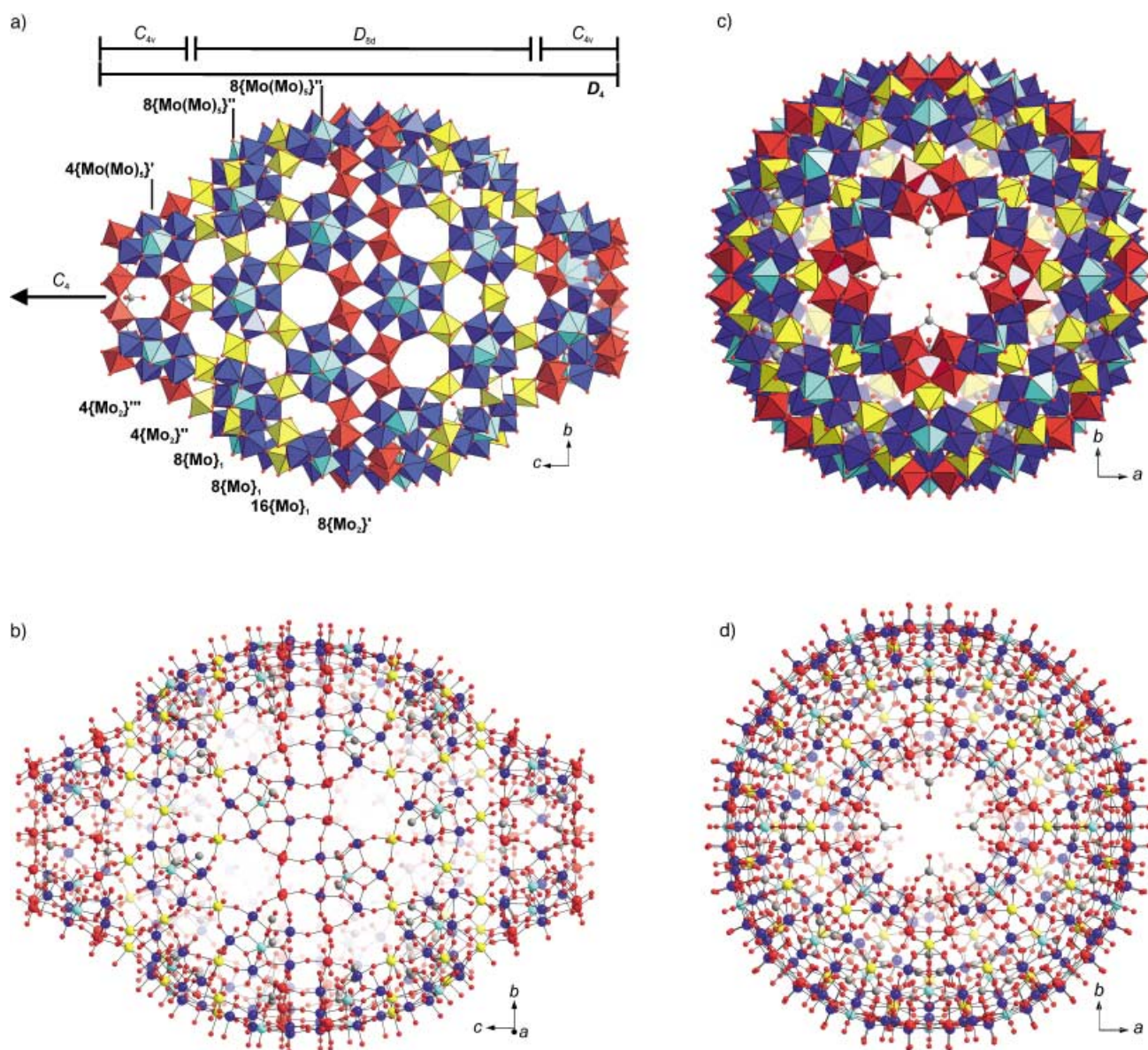
Figure 2. Structure of 1a in crystals of 1 in polyhedral (a) and ball and stick (b) representation perpendicular to the C_4 axis and along the C_4 axis ((c) and (d); building units \{\text{Mo}_1\} yellow, \{\text{Mo}_2\} red, \{\text{Mo}(\text{Mo}_5)\} blue with blue-turquoise pentagonal bipyramids; O atoms small red spheres, S atoms gray spheres). Note that one capping part is turned against the other by 360/16^\circ . The different building blocks and the arrays of different local symmetry are assigned.
